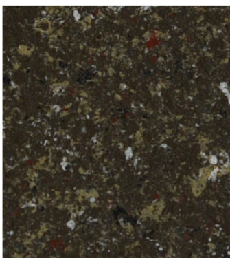
708 Telluride
