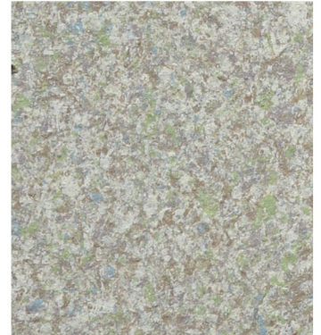
251 Clay
